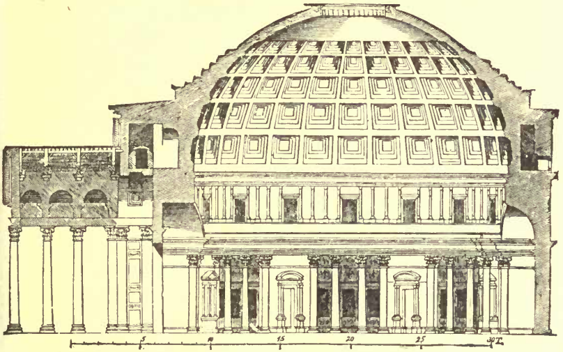
SECTION OF THE PANTHEON
